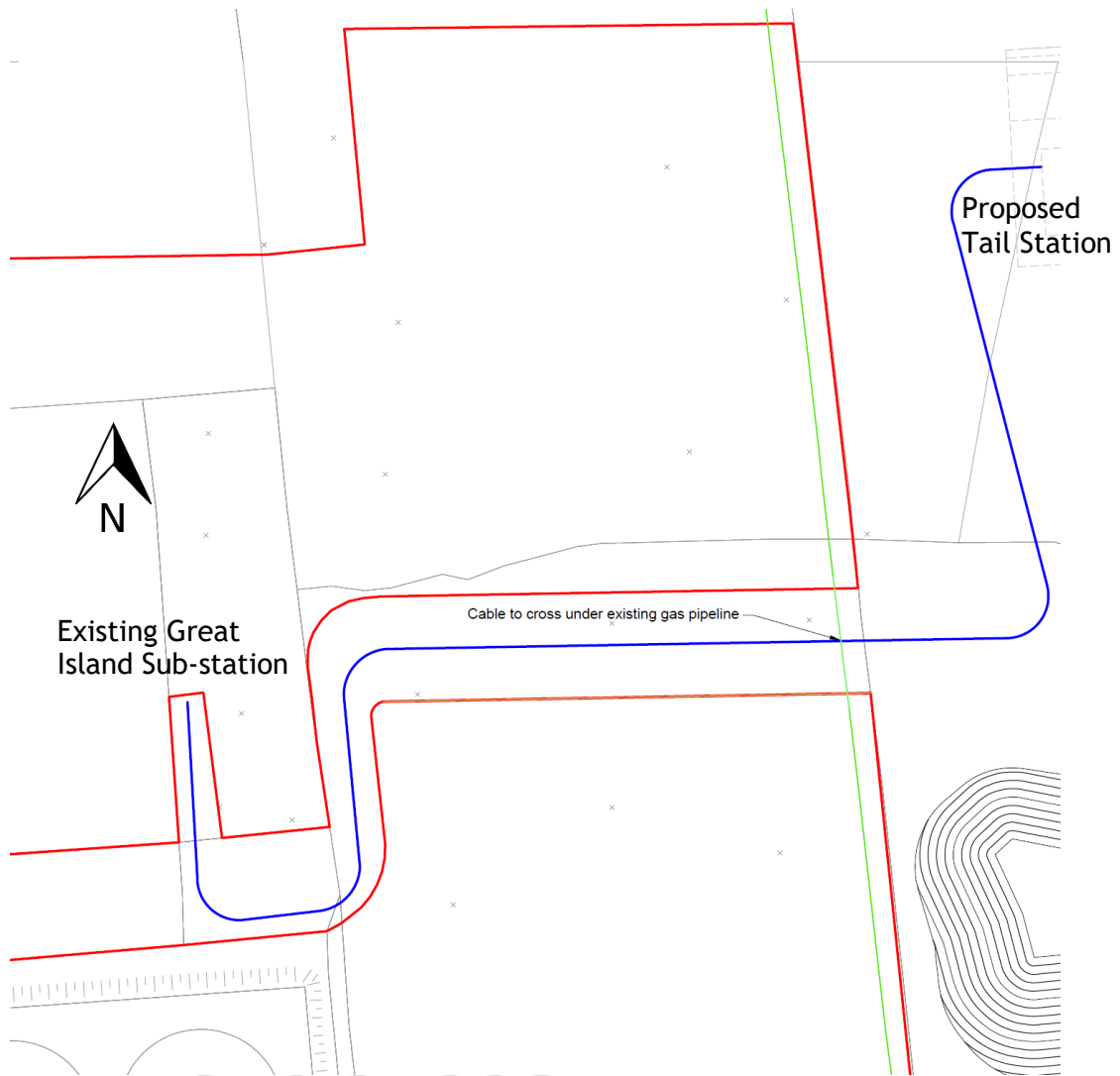
Figure 3.1: HVAC Cable Route (blue line) | not to scale
