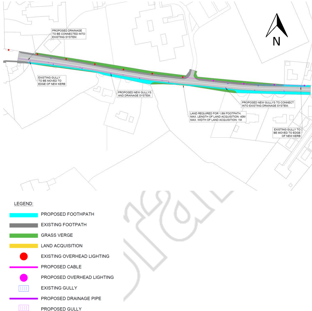
Figure 3.20: Proposed Pedestrian Amenity Improvement Works at Ramsgrange | not to scale
